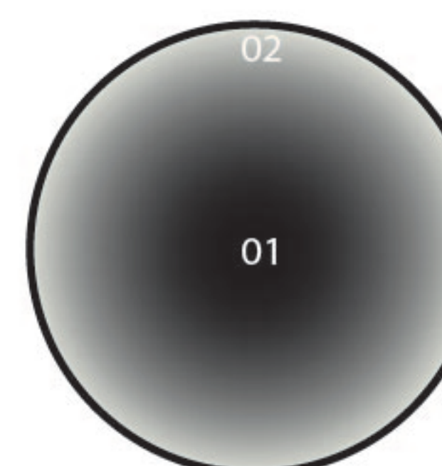
Mammatus
