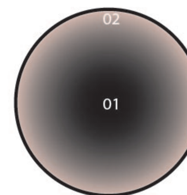
Mammatus
