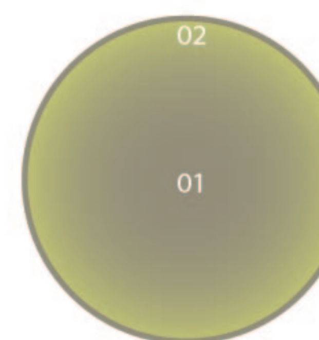
Mammatus
