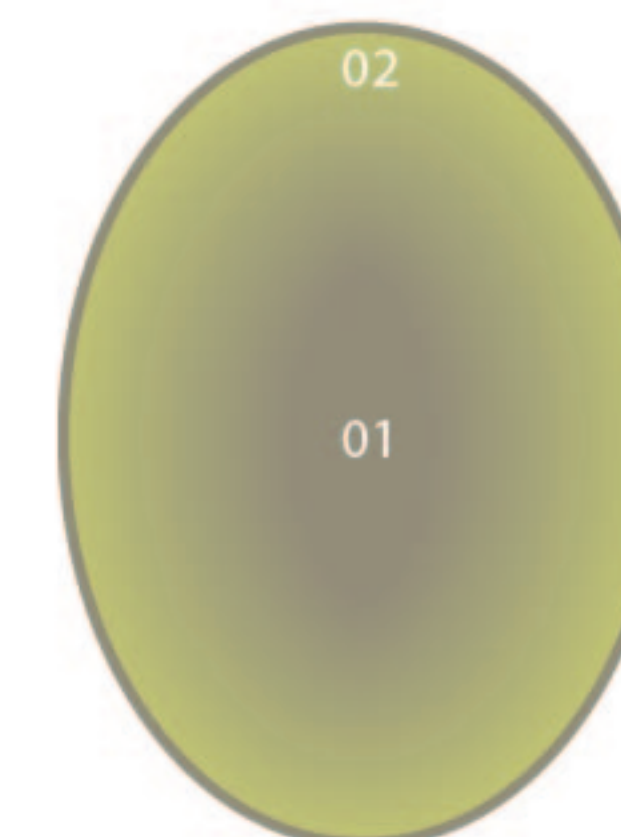
Isobarus
