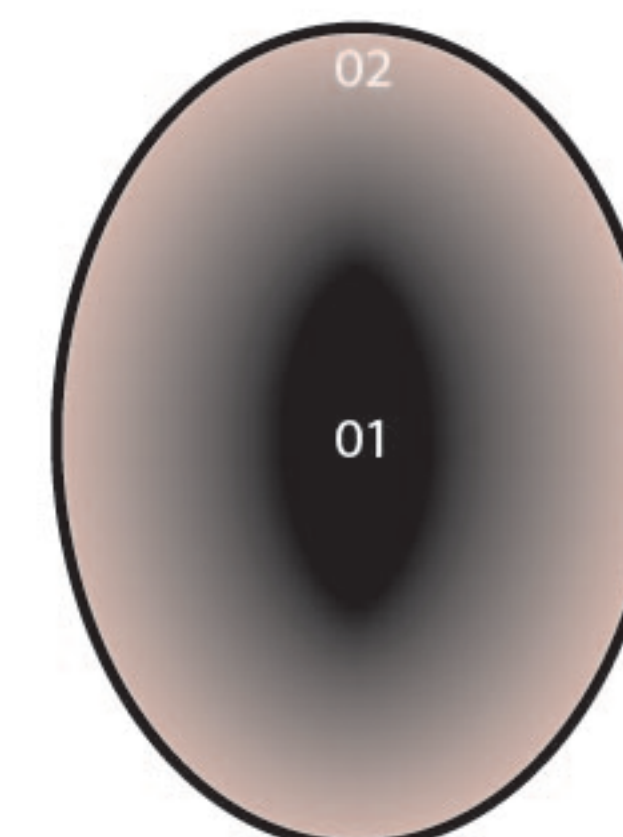
Isobarus
