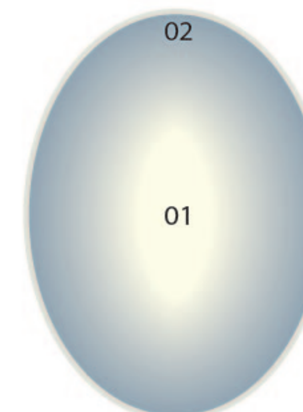
Isobarus
