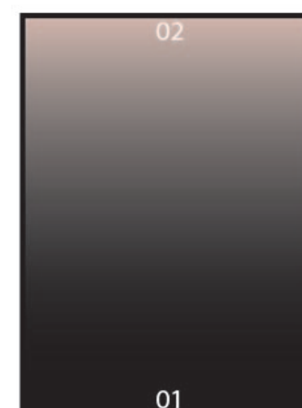
Stratus
