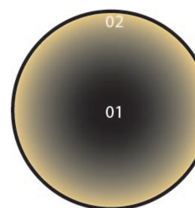
Mammatus
