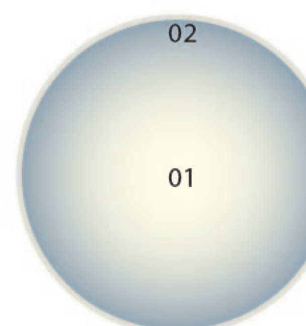
Mammatus
