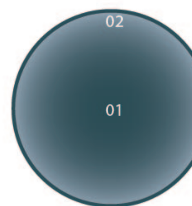
Mammatus
