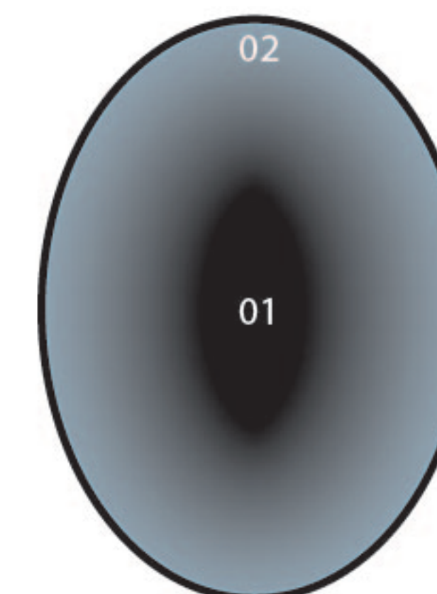
Isobarus
